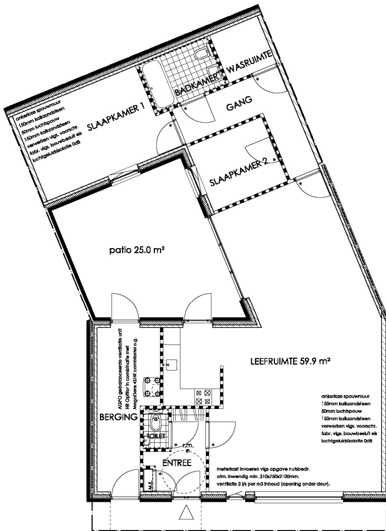
beganegrond bungalow 19
